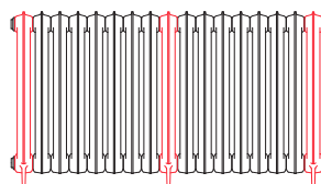
920 x 1426 17 sections (3+14)
