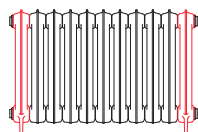
720 x 934 11 sections (2+9)
