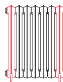
920 x 606 7 sections (2+5)
