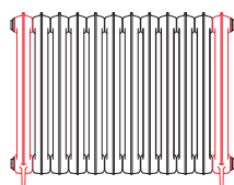
920 x 1016 12 sections (2+10)
