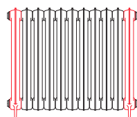
920 x 934 11 sections (2+9)
